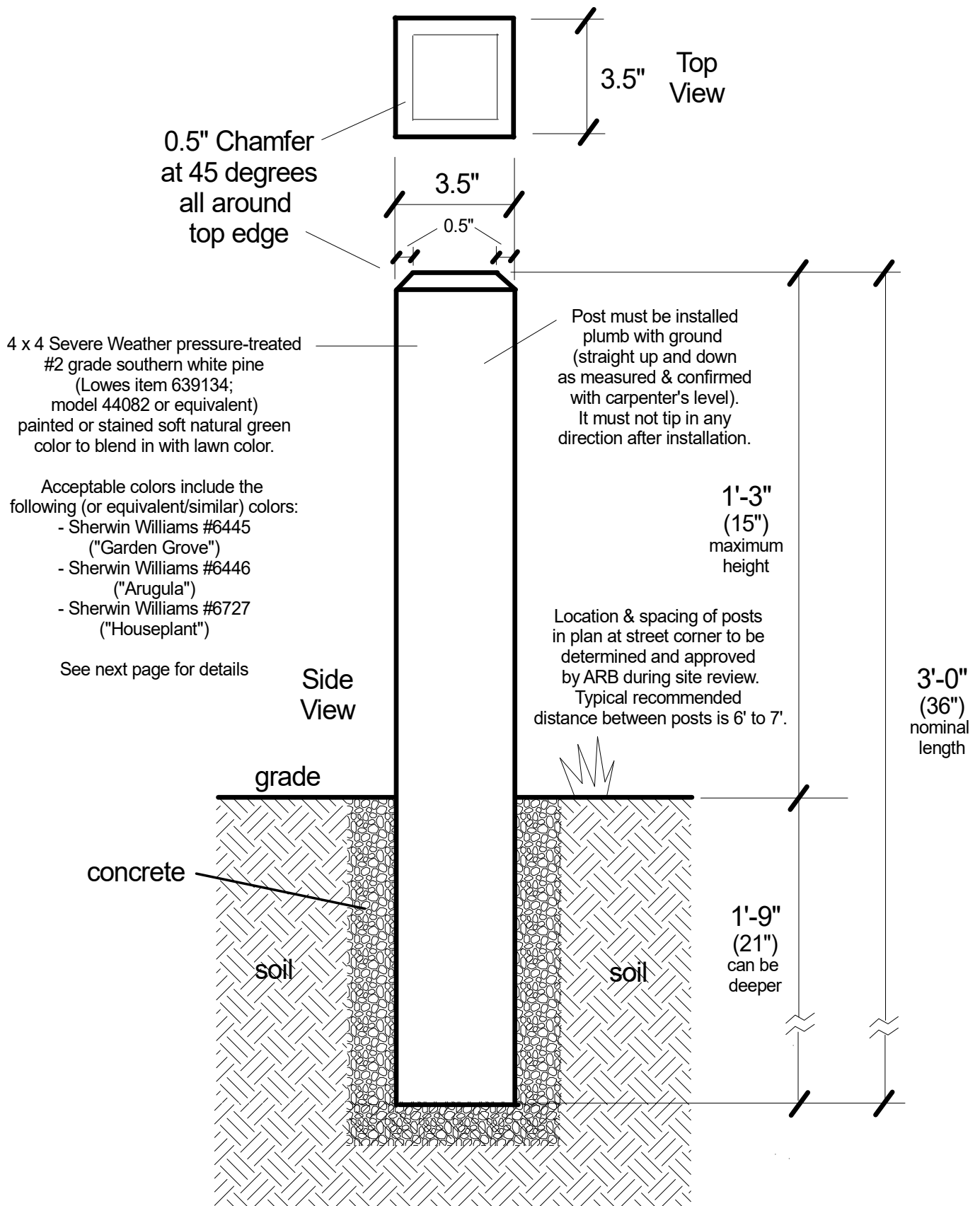
ARB-approved Post design for curb drive-over protection scale: 3"=1'-0"
